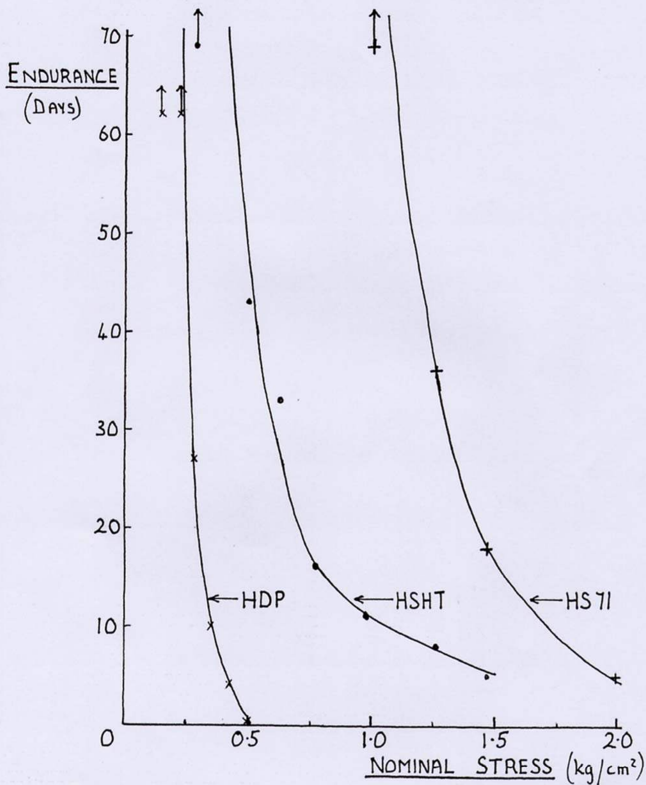
FIG. 2. CREEP RESULTS.
